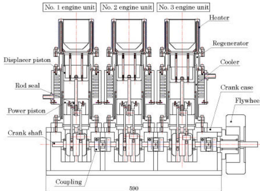
Fig. 9, Schematic View of the Prototype Stirling Engine
