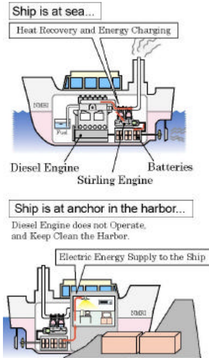
Fig. 6, Waste Heat Recovery System to Keep Clean the Harbor Area
