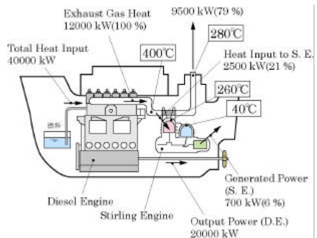
Fig. 5, Energy Balance of Heat Recovery System for Large Ship
