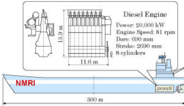
Fig. 1, Marine Diesel Engine for Large Freight Ship
