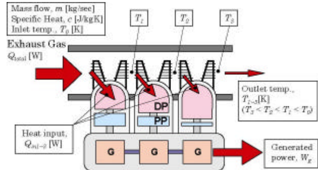
Fig. 7, Concept of Multi-cylinder Stirling Engine
