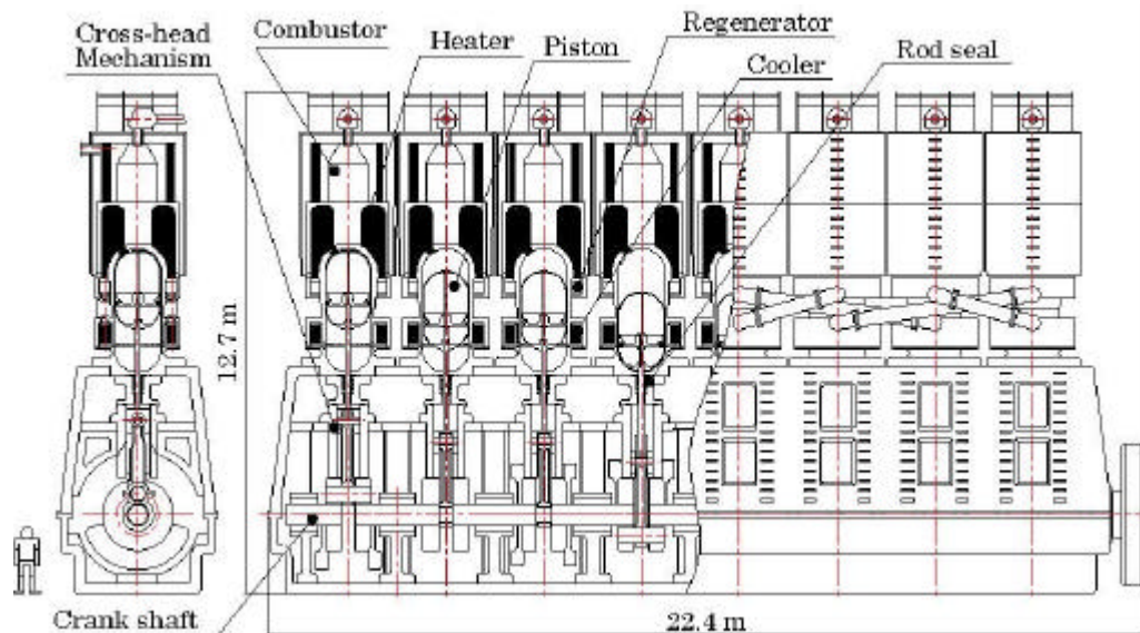
Fig. 3, Conceptual Drawing of the 20,000 kW class Marine Stirling Engine
