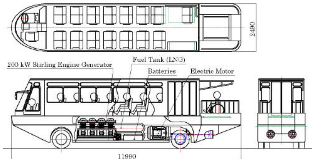
Fig. 4, Conceptual Drawing of Sightseeing Amphibious Vehicle
