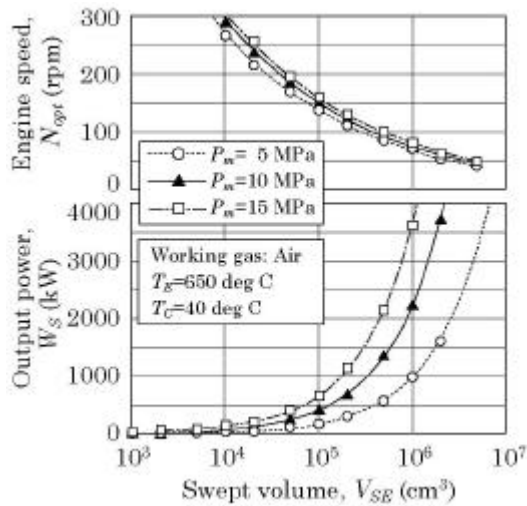
Fig. 2, Calculated Results of Stirling Engine Performance by Simple Prediction Method
