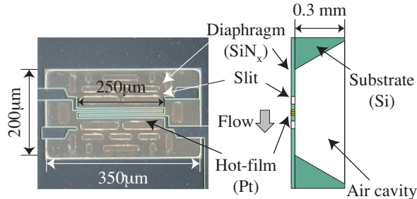
Fig. 10 Magnified view of micro hot-film shear stress sensor presently developed (Type 2).
