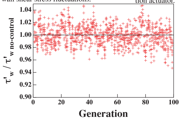
Fig. 7 Feedback control results using the 1st generation control system. Root-mean-square value of the wall shear stress fluctuations is plotted versus generation of GA-based control algorithm.
