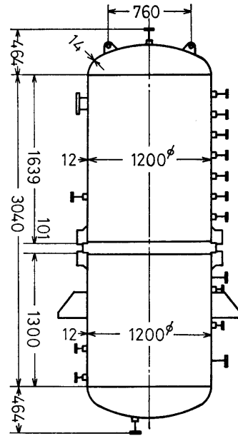
図 3-5 Containment Details
