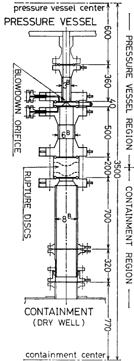
図 3-7 Discharge Line Details
