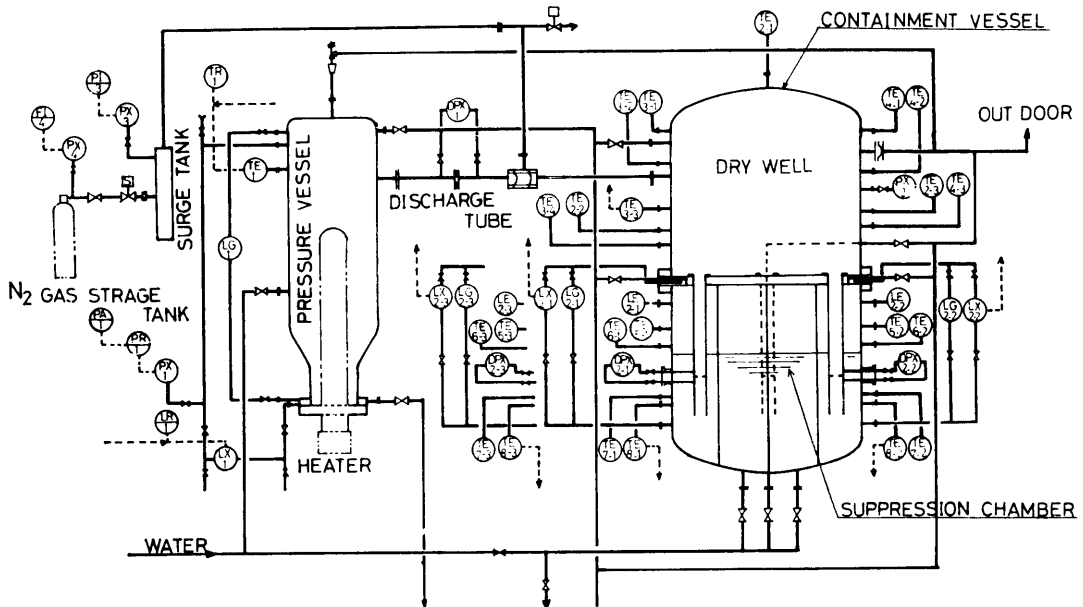
図 3-2 Flowsheet of Experimental Equipment
