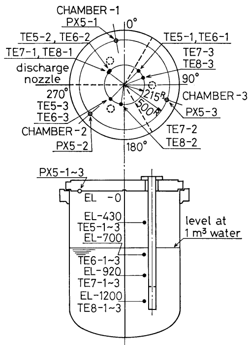
図 3-9 Location of Thermocouples and Pressure Pickups in Wetwell
