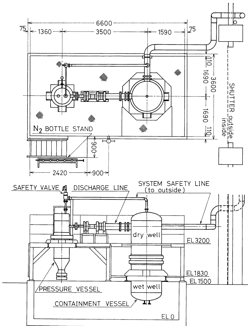
图 3-3 Experimental System Outline
