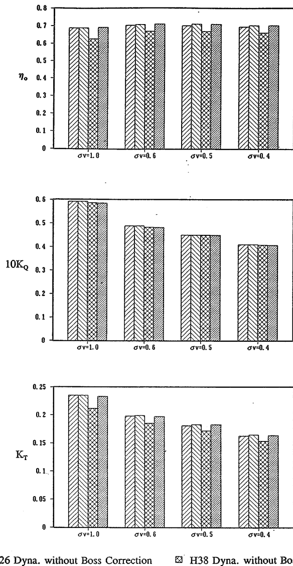
SRIJ-II Propeller J=1.1
