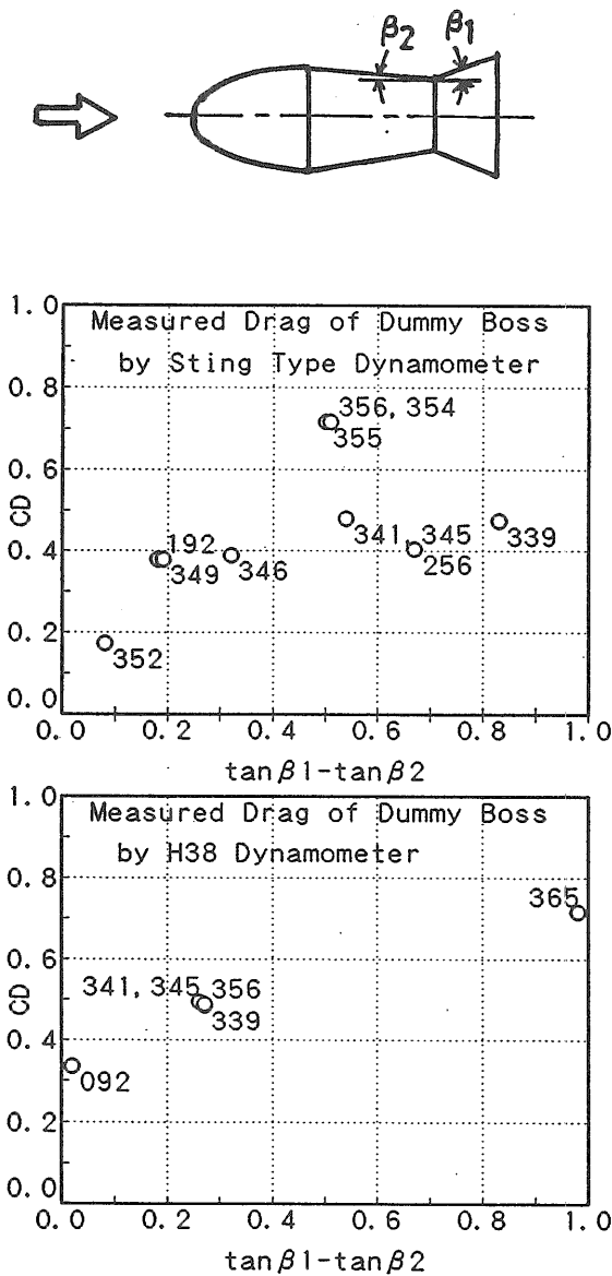
Fig. 5.4 Relationship between Resistance and Shape of Boss for Two Kinds of Dynamometers
