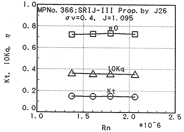
Fig. 4.30 (b) Viscous Effect on SRIJ-III Propeller Performance Measured by Using J26 Dynamometer
