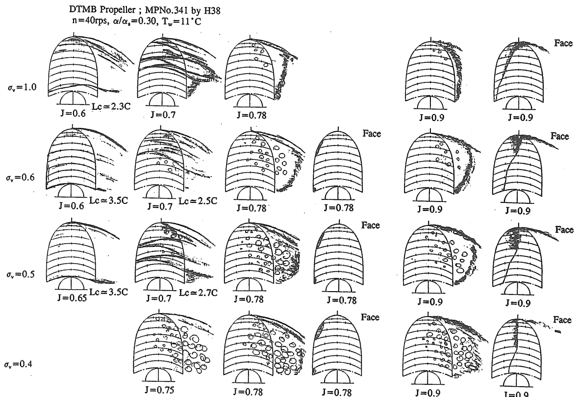
Fig. 4.17 Sketch of Cavitation Pattern on DTMB Propeller Set up to H38 Dynamometer
