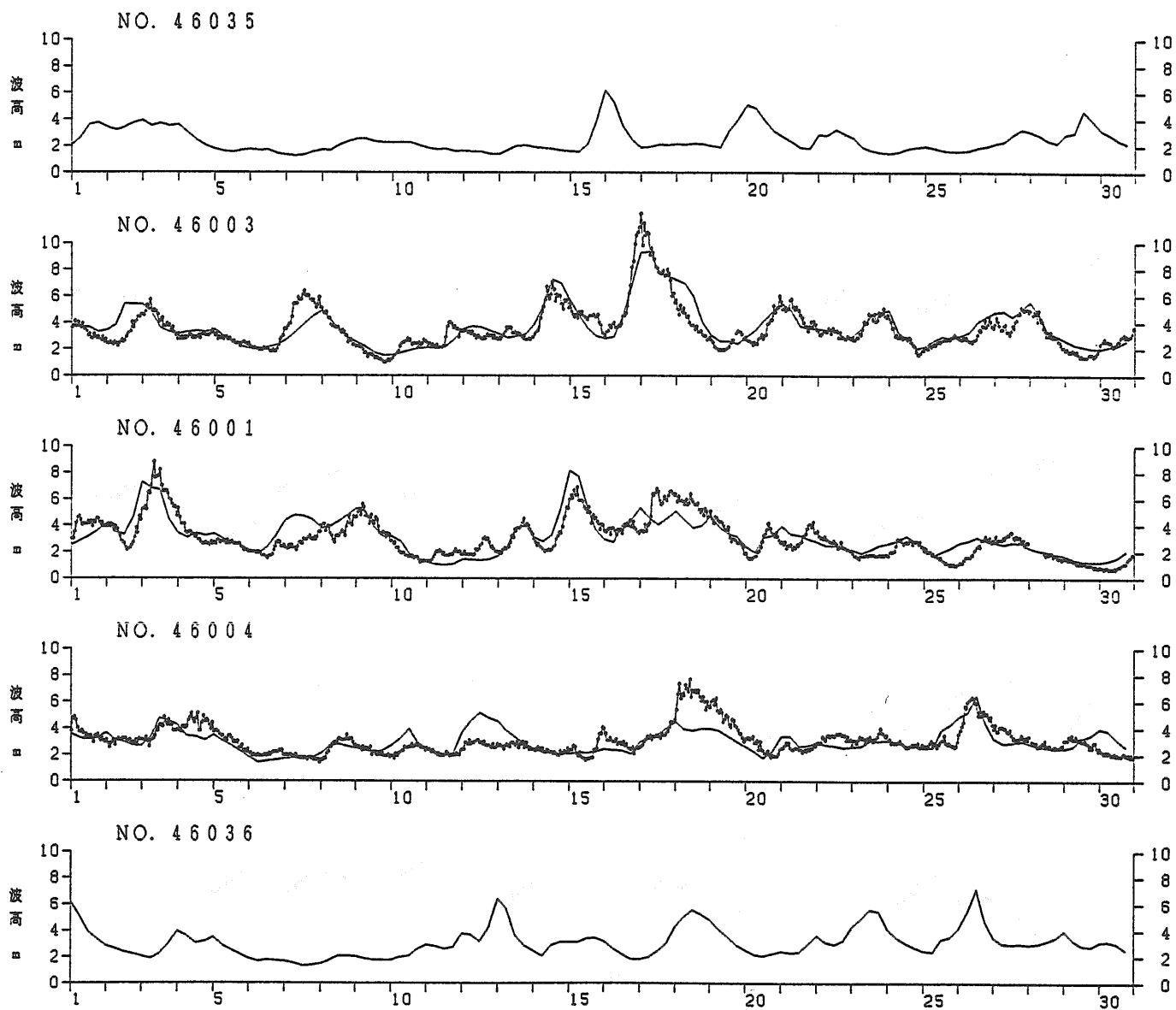
Fig. 1. 6. 5 Comparison of Hindcasted Wave Heights with NOAA Buoy Data April, 1985
