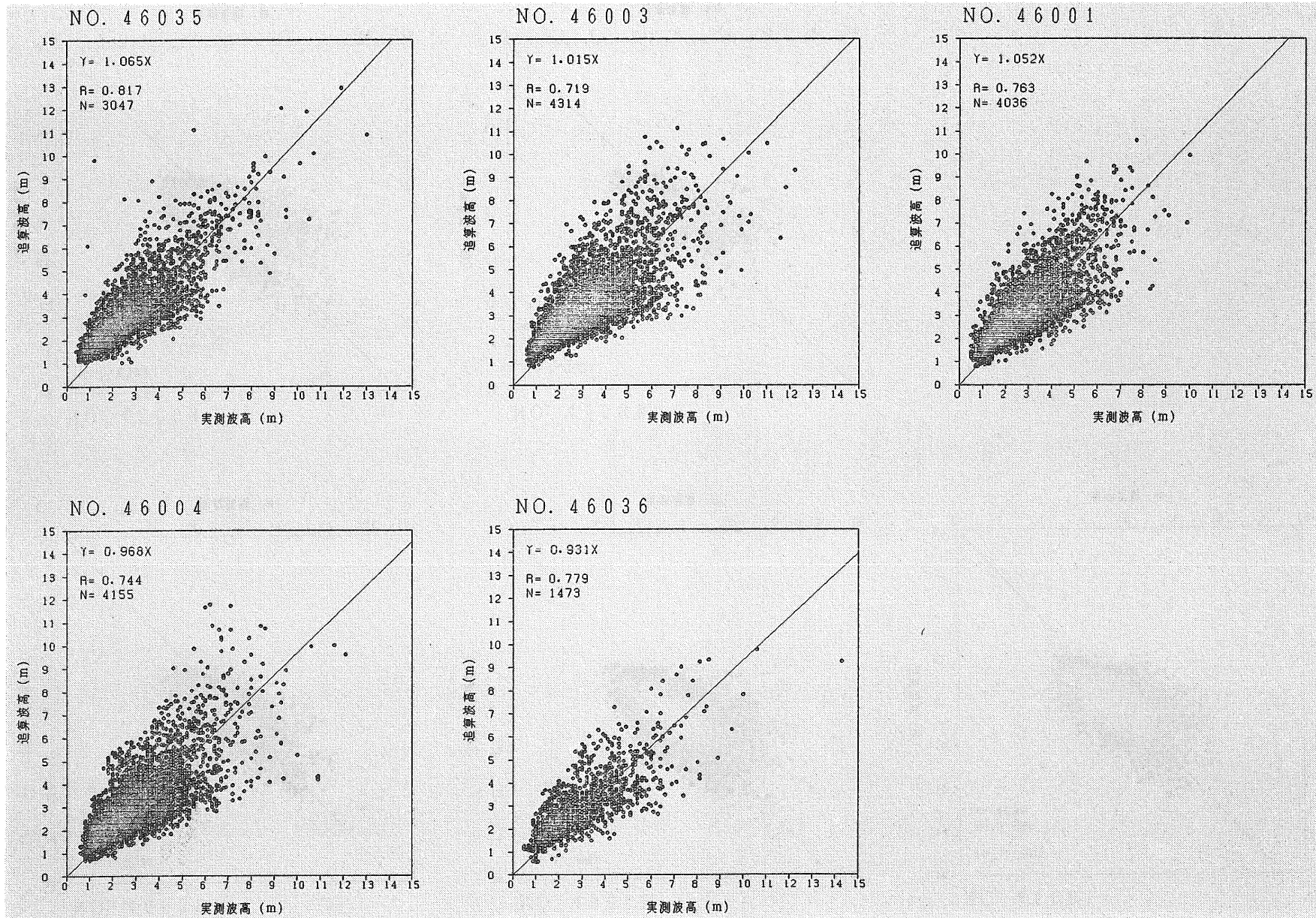
Fig. 1. 8. 2 Correlation between Hindcasted and NOAA Buoy Data Wave Height
