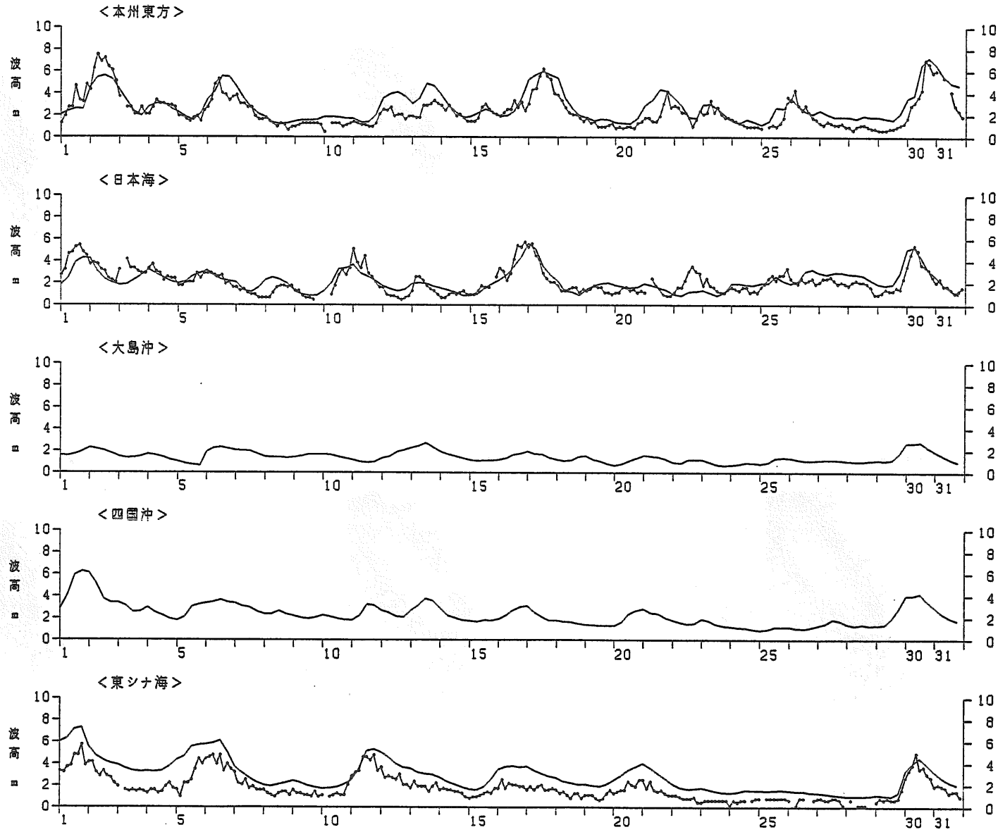
Fig. 1. 7 Comparison of Hindcasted Wave Heights with JMA Buoy Data
