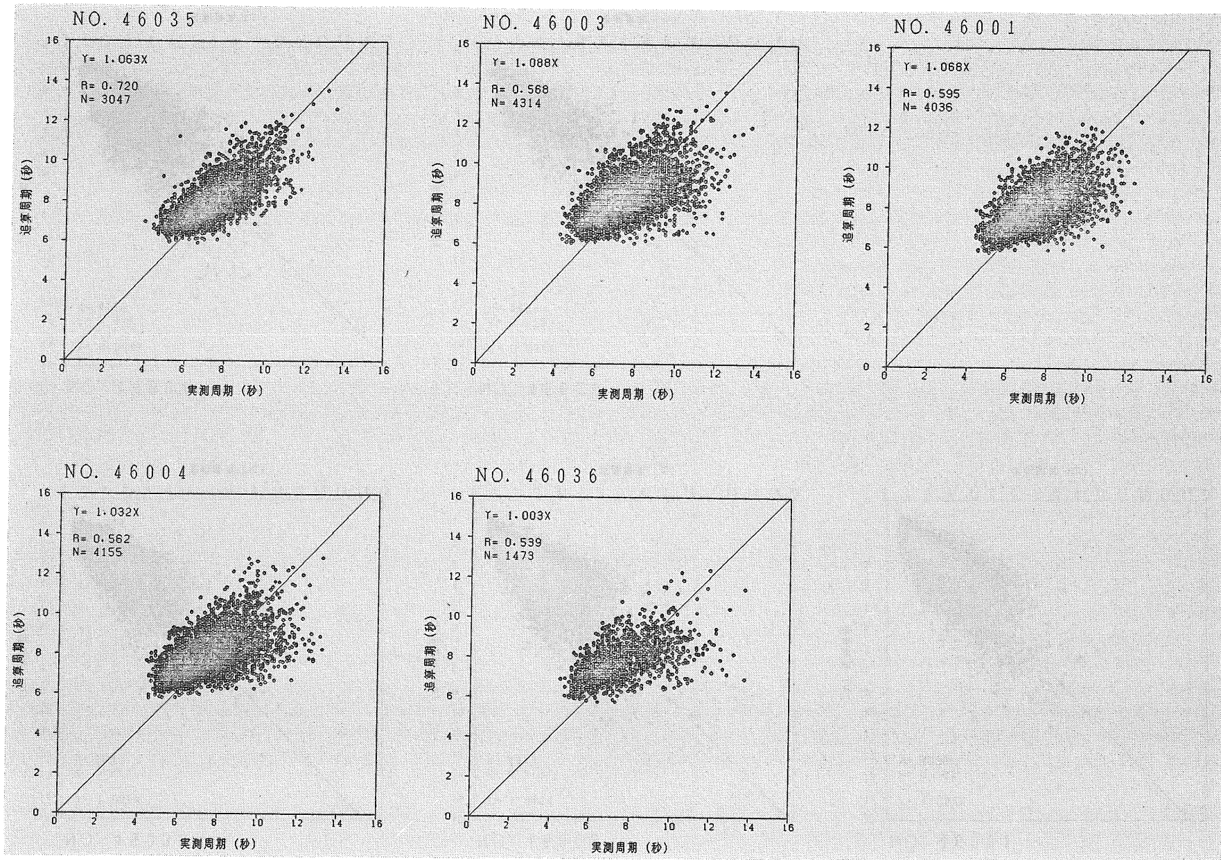
Fig. 1.8.3 Correlation between Hindcasted and NOAA Buoy Data Wave Period
