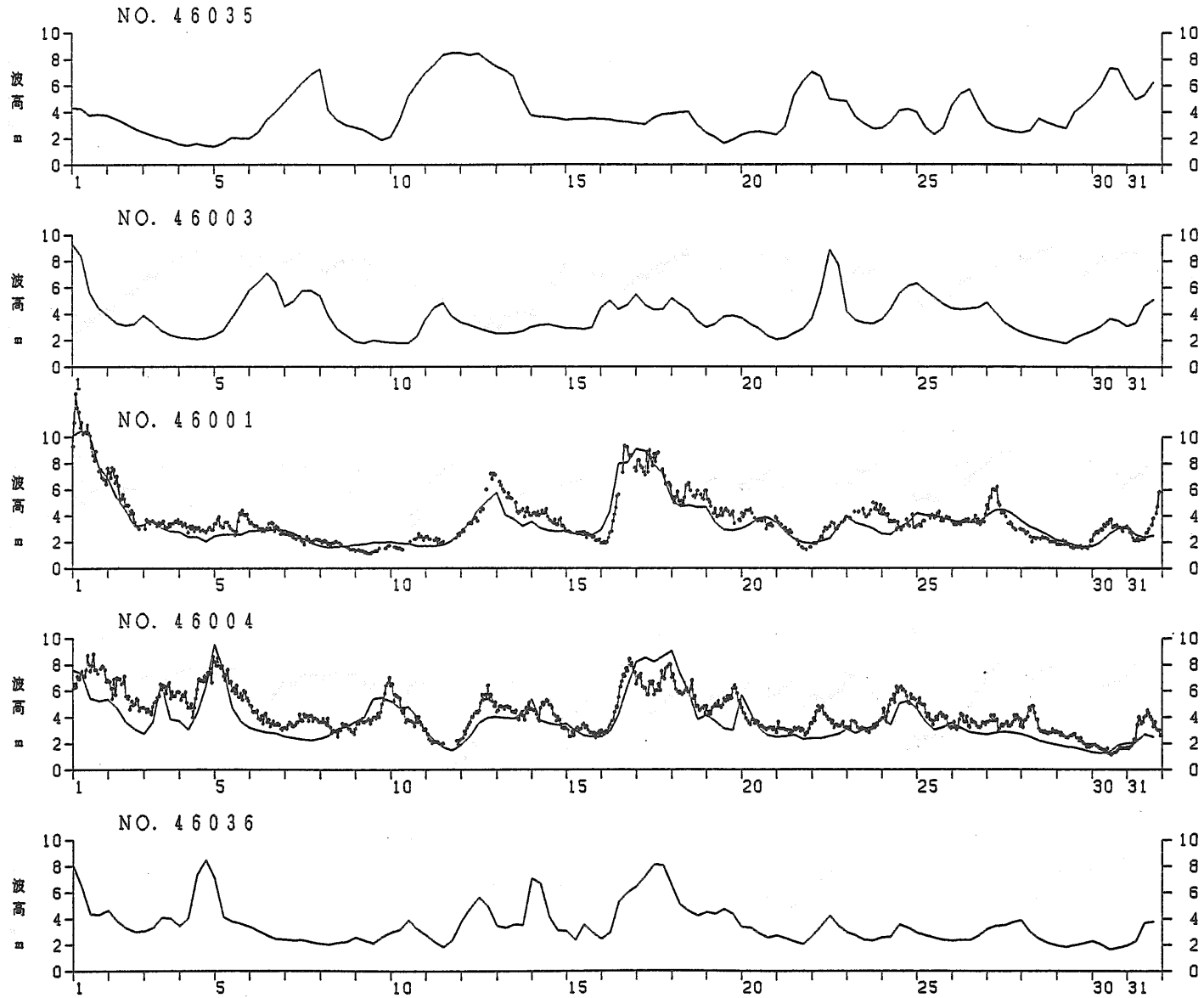
Fig. 1.6.3 Comparison of Hindcasted Wave Heights with NOAA Buoy Data December, 1981
