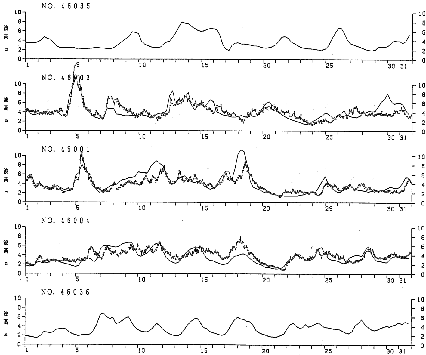
Fig. 1. 6. 1 Comparison of Hindcasted Wave Heights with NOAA Buoy Data March, 1981
