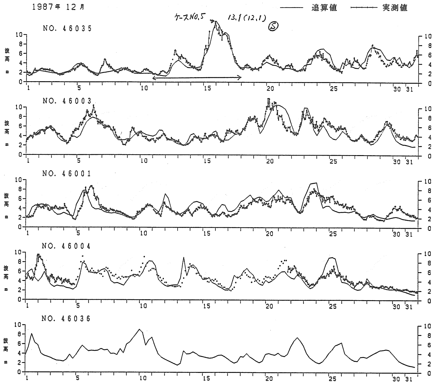
Fig. 1. 6. 6 Comparison of Hindcasted Wave Heights with NOAA Buoy Data December, 1987
