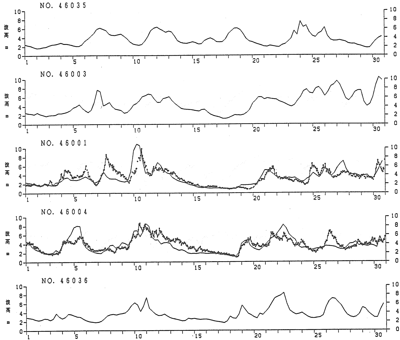
Fig. 1.6.2 Comparison of Hindcasted Wave Heights with NOAA Buoy Data November, 1981
