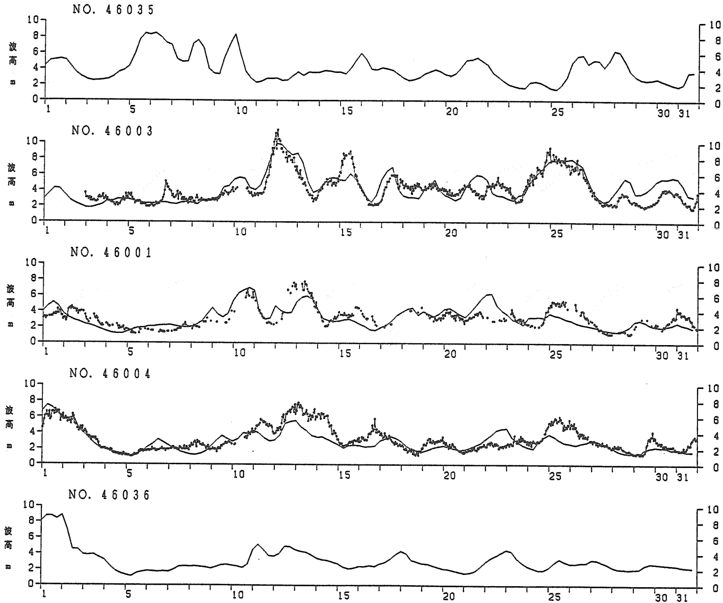
Fig. 1.6.4 Comparison of Hindcasted Wave Heights with NOAA Buoy Data March, 1982
