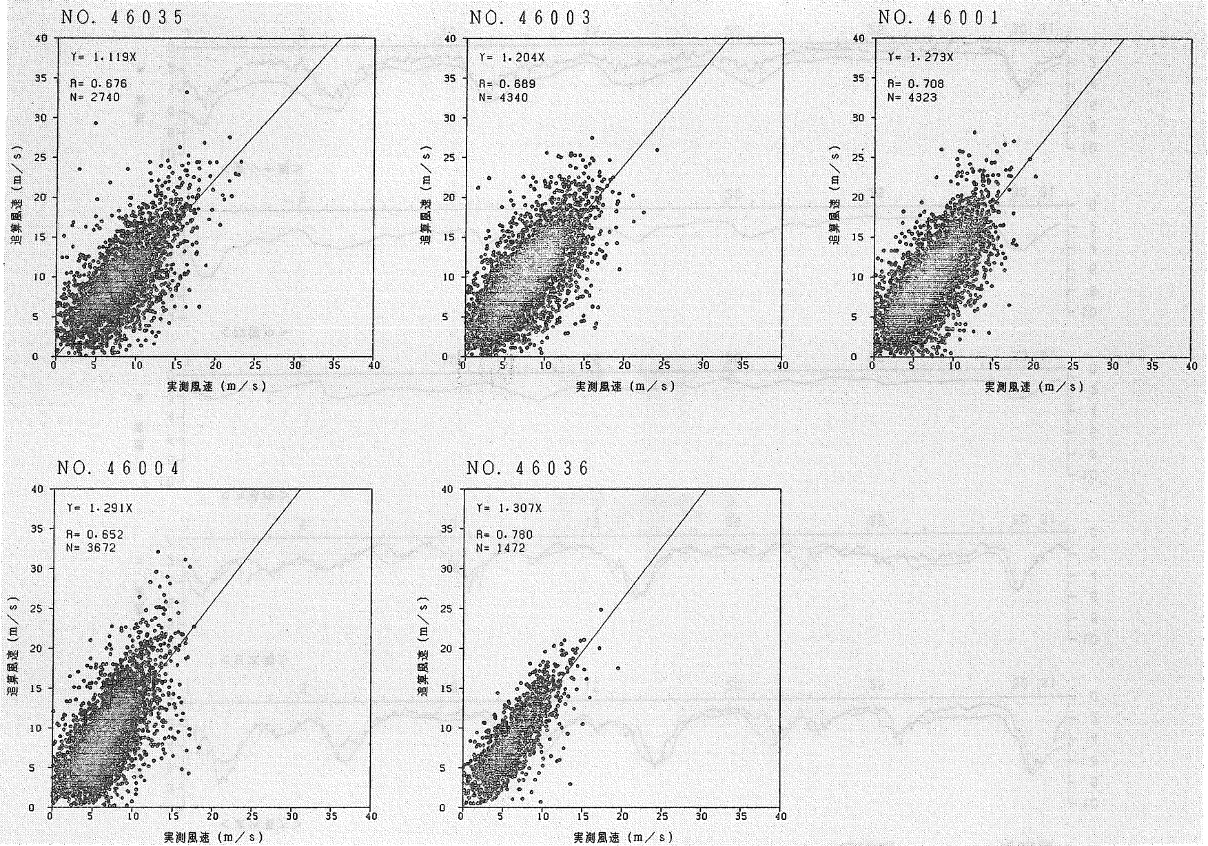
Fig. 1.8.1 Correlation between Hindcasted and NOAA Buoy Data Wind Speed
