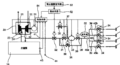
10 Main engine 52 Draw-off means 53 Draw-off level setting means 54 Control means 55 Air reservoir
